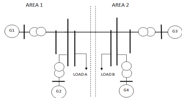
Fig.2 One line diagram of single machine infinite bus
