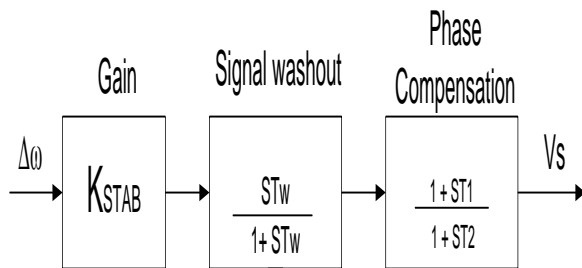
Fig.1 The basic block diagram of CPSS
